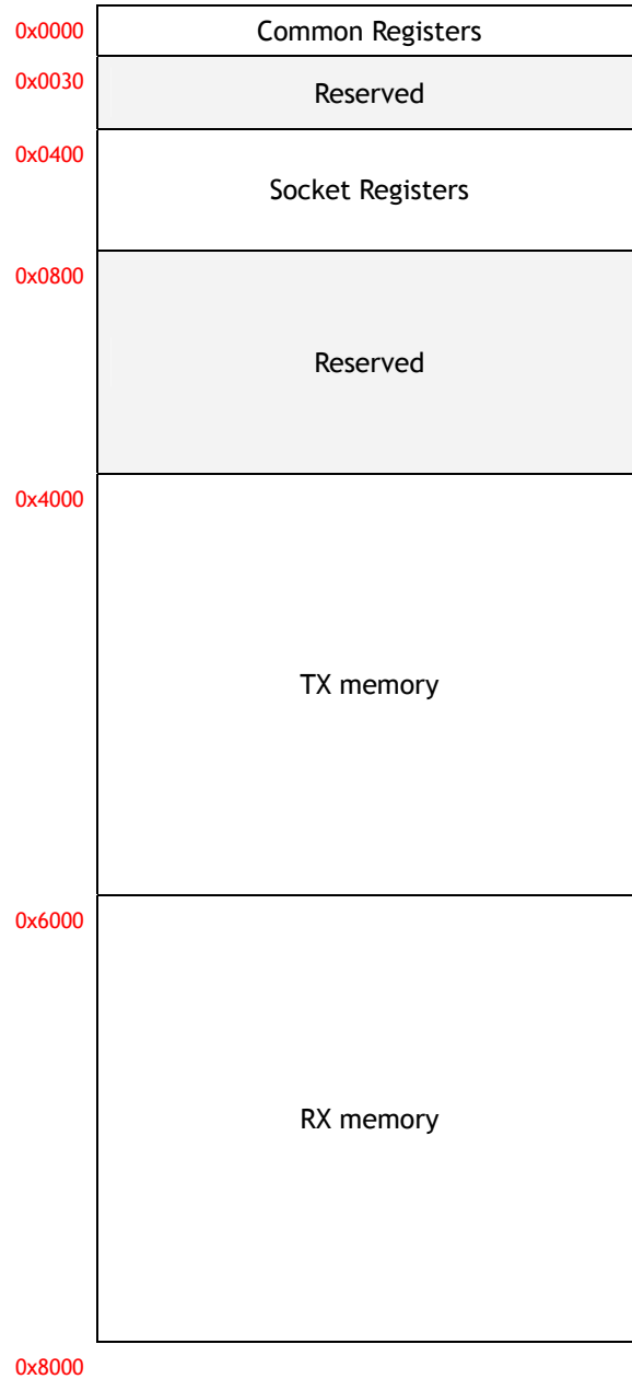
Memory Map
